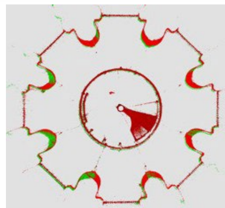
Dio 3D modela Zagrebačke katedrale. Presjek na 85 m – 3.4 cm pomaka (Izvor: Report on the specificity of the situation following two earthquakes in Croatia in 2020.)
