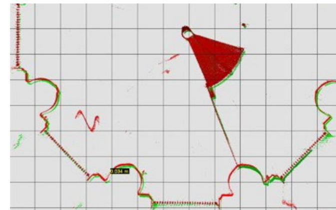
Dio 3D modela Zagrebačke katedrale. Presjek na 85 m – 3.4 cm pomaka (Izvor: Report on the specificity of the situation following two earthquakes in Croatia in 2020.)
